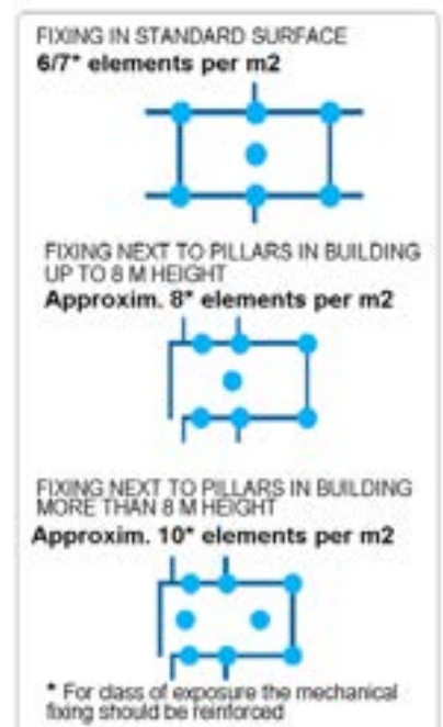
9. Recommendations nr anchors / m^2
