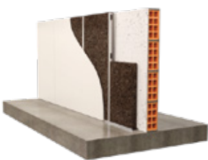
Internal partitions Metal stud over masonry wall with insulation
